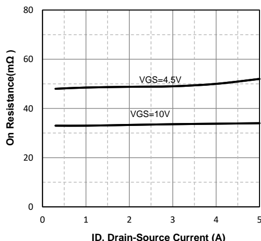
Fig4. On-Resistance Vs. Drain-Source
