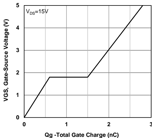
Fig2. Typical Gate Charge Vs. Gate-Source Voltage
